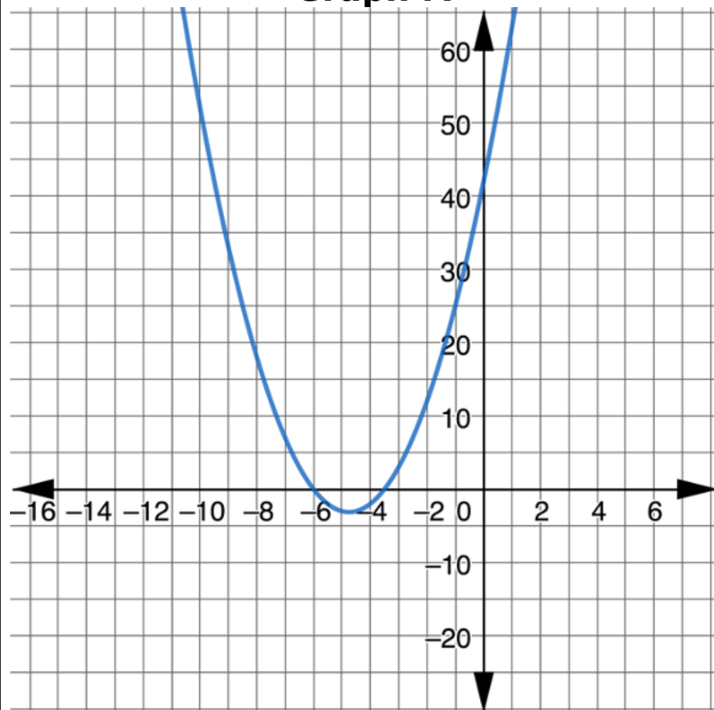
Graph M
