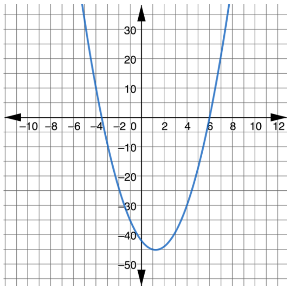
Graph L
